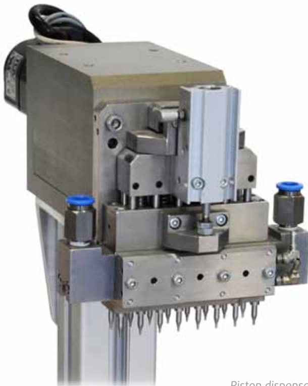
Piston dispenser Dos PM one component, 16 nozzles
