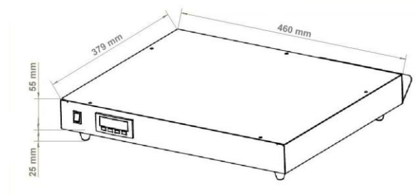
Dimensions of the heater SH 230-1, item number 21001300
